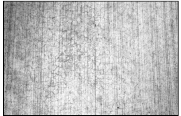
Crazing Concrete Surface (Dampened)
